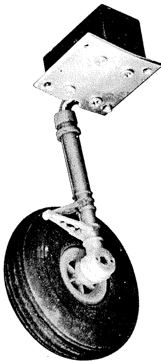
Main landing gear pre-assembly with strut
