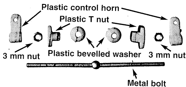
Rudder control hardware
