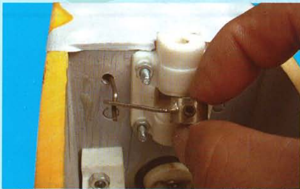
15C- Insert the end of the pre-installed Z-bend wire into the hole in the steering arm
