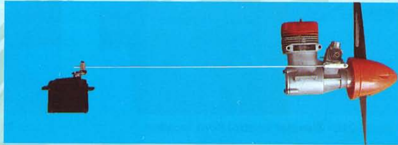
18B- Throttle control rod connected to the engine throttle arm and to the servo arm
