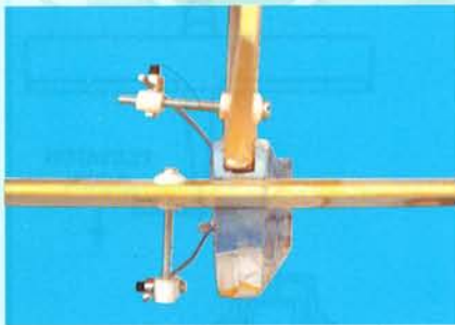
24A- elevator control horn shown in position
