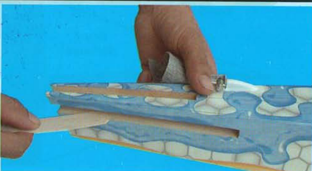
10A- Apply plenty of epoxy
