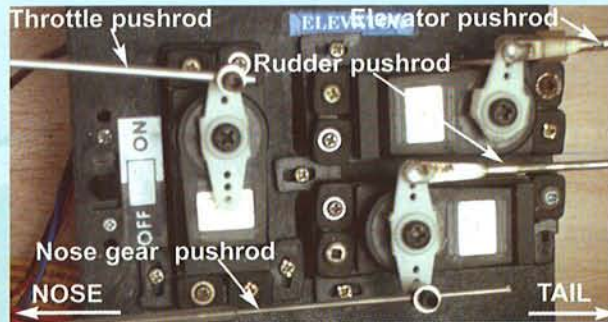
23C- Center the servos, control surfaces & throttle (carb) then connect the control rods to the servos.
