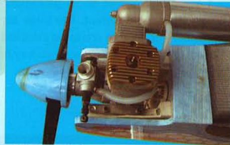
19A- Fuel line connected to the carburetor and pressure line connected to the muffler.
