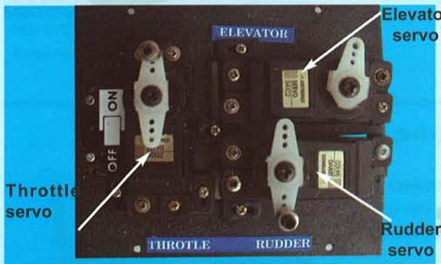
22B- Note the orientation and positions of the three servos in the servo tray
