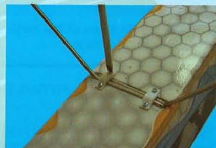
14D- Use 4 sheet metal screws and 2 straps to mount the main landing gears onto the fuselage
