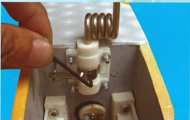
15E- Insert the nose gear into the bearing, passing through the steering arm. Secure the steering arm to the nose gear by tightening the set screw onto the flat spot on the nose gear wire.
