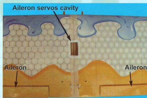
4B- Aileron servo location
